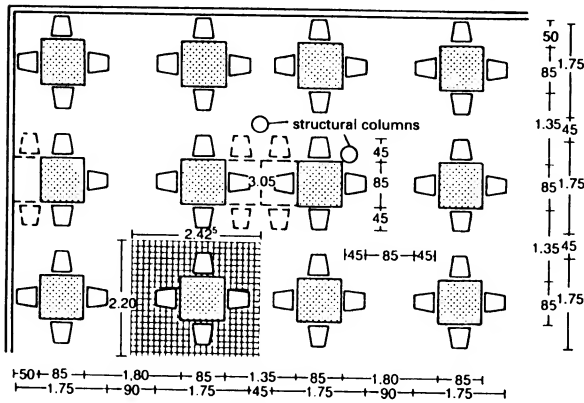
③ Parallel table arrangement
